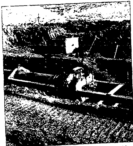
Laying the Land-Based Gas Line – First Stage. July 2006.
